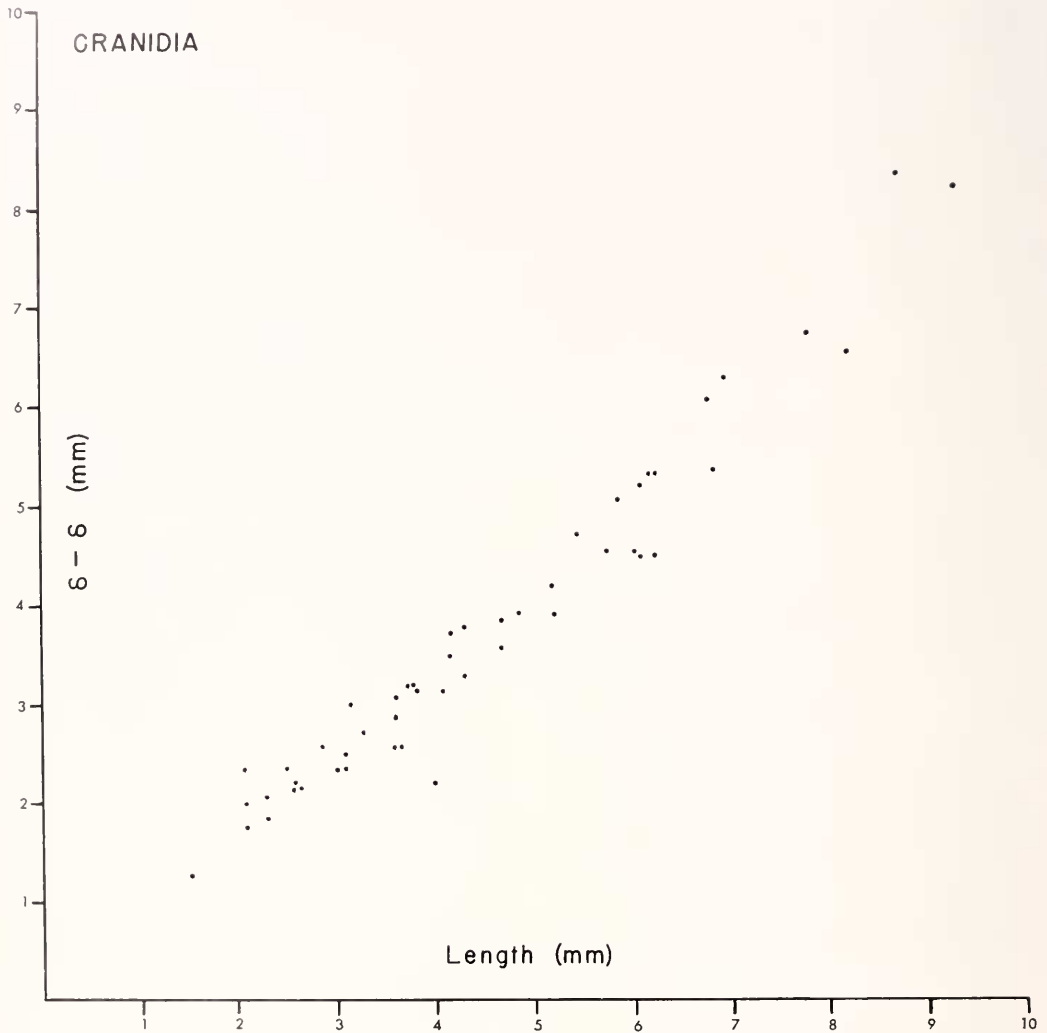
Figure 2. Proetus pluteus n. sp. Dimensions of 50 cranidia; length is sagittal; \delta - \delta is width across palpebral lobes at widest point. Measured cranidia include USNM 154458-60, 154464-6, 154475, 154478, figured specimens, remainder included under 154489.
